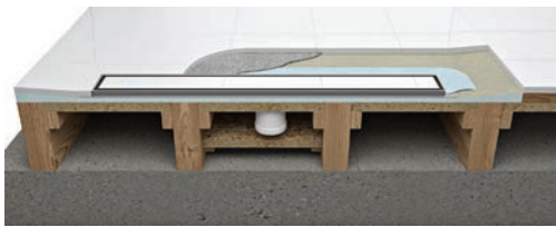
Tray & Drain using underboarding, including under trap
