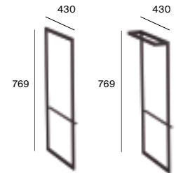
Optional furniture legs (reversible) 769mm for 2 drawer furniture
