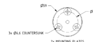
2x MOUNTING PLATES
