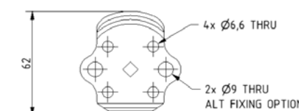
WALL FIXING PLATE
