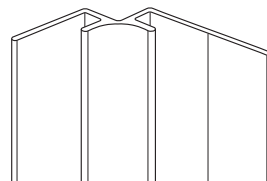
Internal Corner Use these profiles when needing to join two panels on an internal joint.
