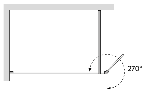
WETROOM FRONT PANEL WITH DEFLECTOR PANEL
