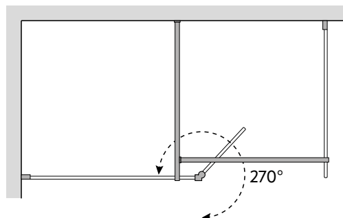
WETROOM FRONT AND SIDE PANEL WITH DEFLECTOR PANEL
