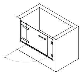
Wall Hinge Door with Two Inline Panels in Recess
